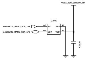
MAGNETIC SENSOR
