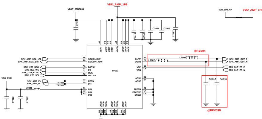
SPK AMP
