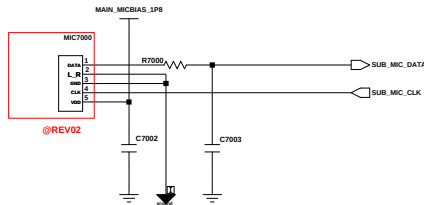
2nd MIC
