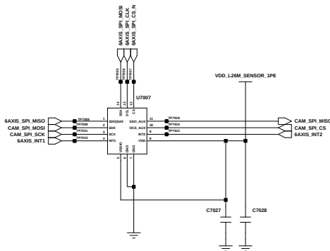
ACC&GYRO SENSOR
