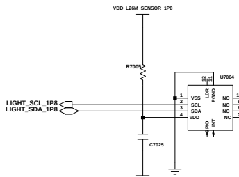
AMBIENT SENSOR
