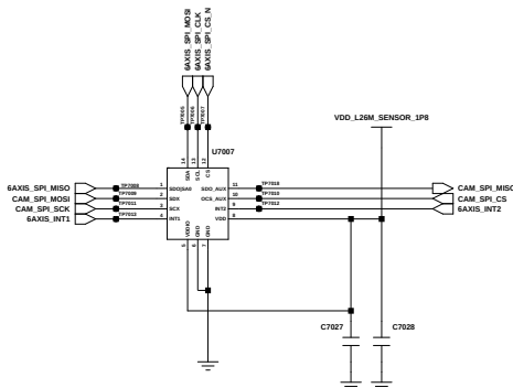
ACC&GYRO SENSOR
