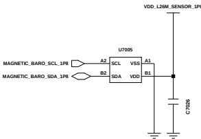
MAGNETIC SENSOR
