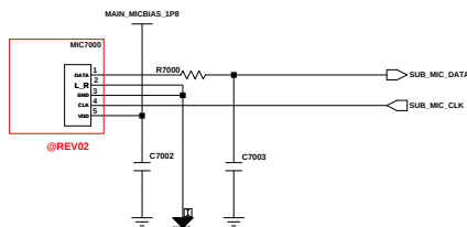
2nd MIC
